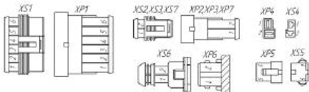
Figure 4.1- Wiring Diagram
